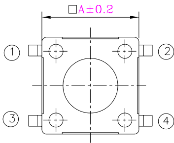
P.C.B. HOLE DETAIL
