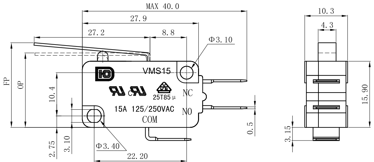
SCHMATIC
